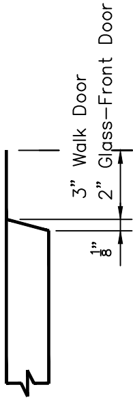
Side View at Head Trim
